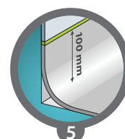
5 Heat-sealed joint with flexible flooring
