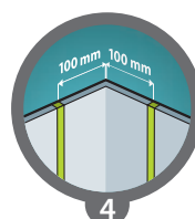
4 Thermoformed internal corners
