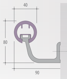
Aluminium mounting bracket
